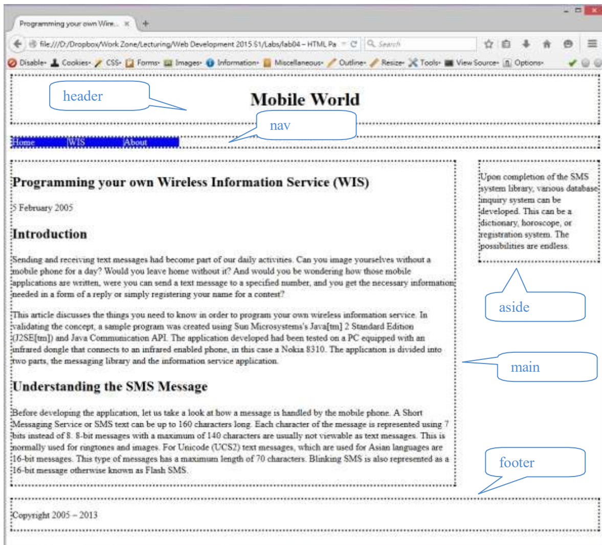
Figure 1. Styled webpage wis.html
